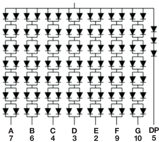
COMMON ANODE 1 & 8
